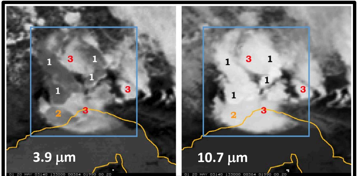
GOES-12 3.9 \mu\text{m} Brightness Temperatures (BTs) (Left) and 10.7 \mu\text{m} BTs. Ice Crystal Size at anvil top affects the amount of reflected solar radiation at 3.9 \mu\text{m} and consequently the BT, displayed as a greyscale, with whites cold and blacks hot. 10.7 \mu\text{m} BTs are less affected by Ice Particle Size. (Credit: Chad Gravelle, CIMSS/OPG)
